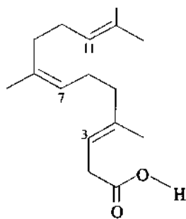
3,7-trans/ cis- isomer
